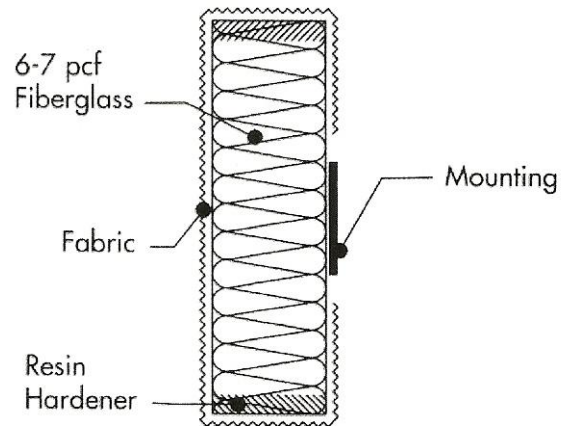
Core Section
